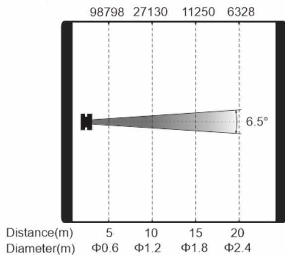
Intensity LUX(6.5°)
