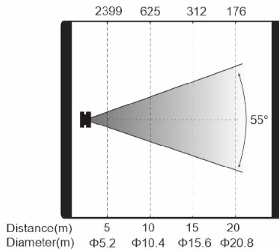
Intensity LUX (55°)
